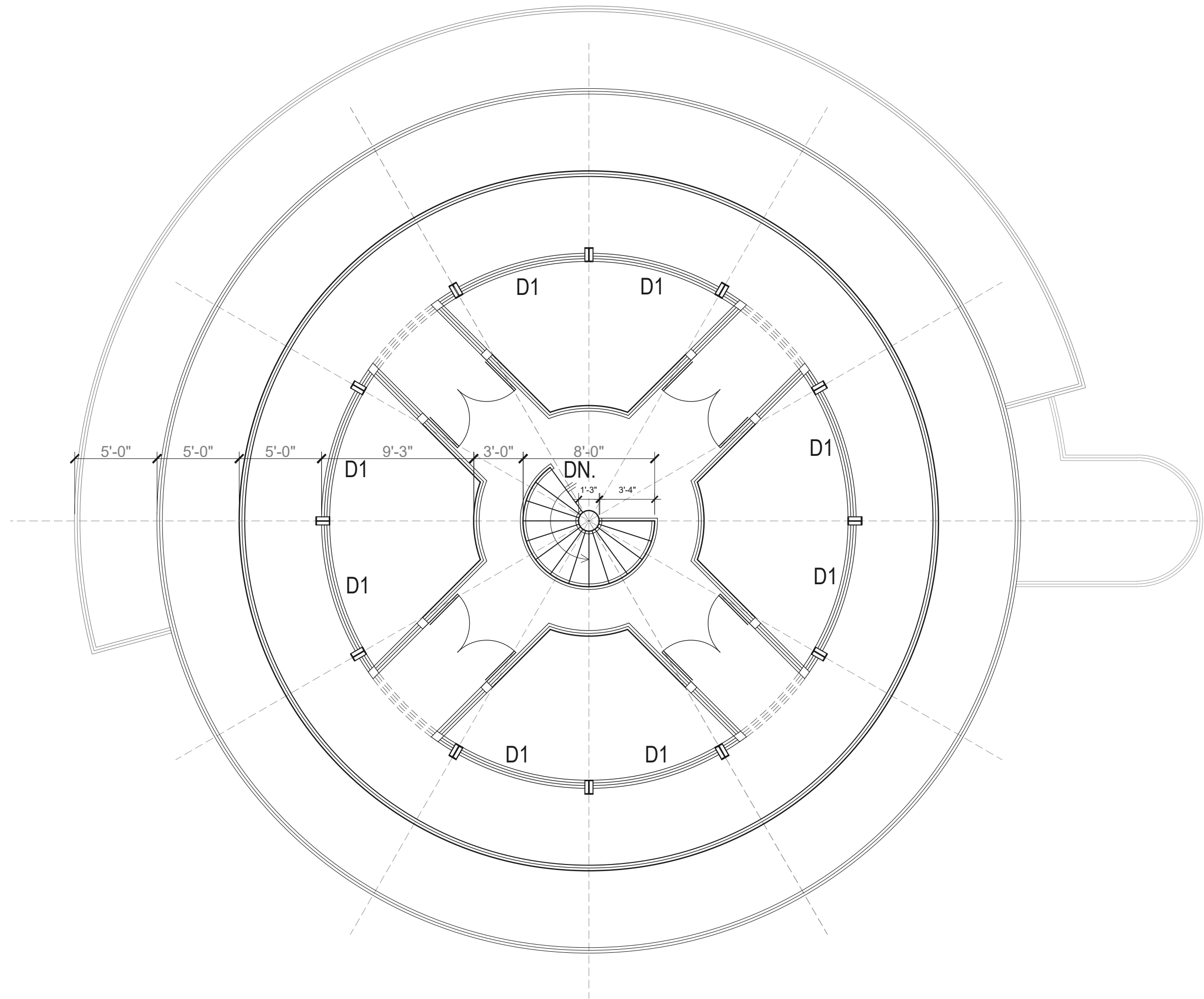
THIRD FLOOR PLAN SCALE = 3/8" = 1'-0"
