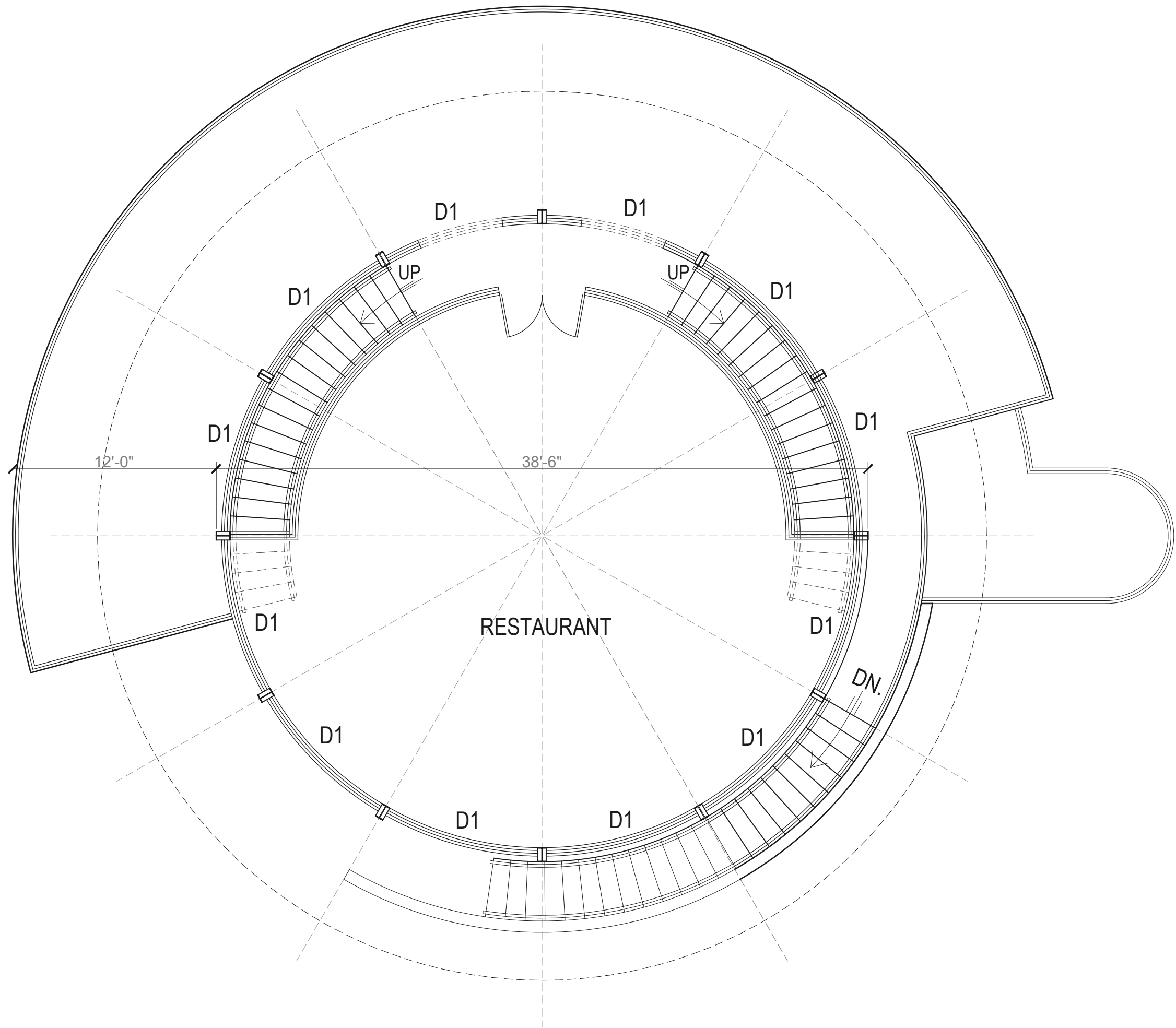
FIRST FLOOR PLAN SCALE = 3/8" = 1'-0"
