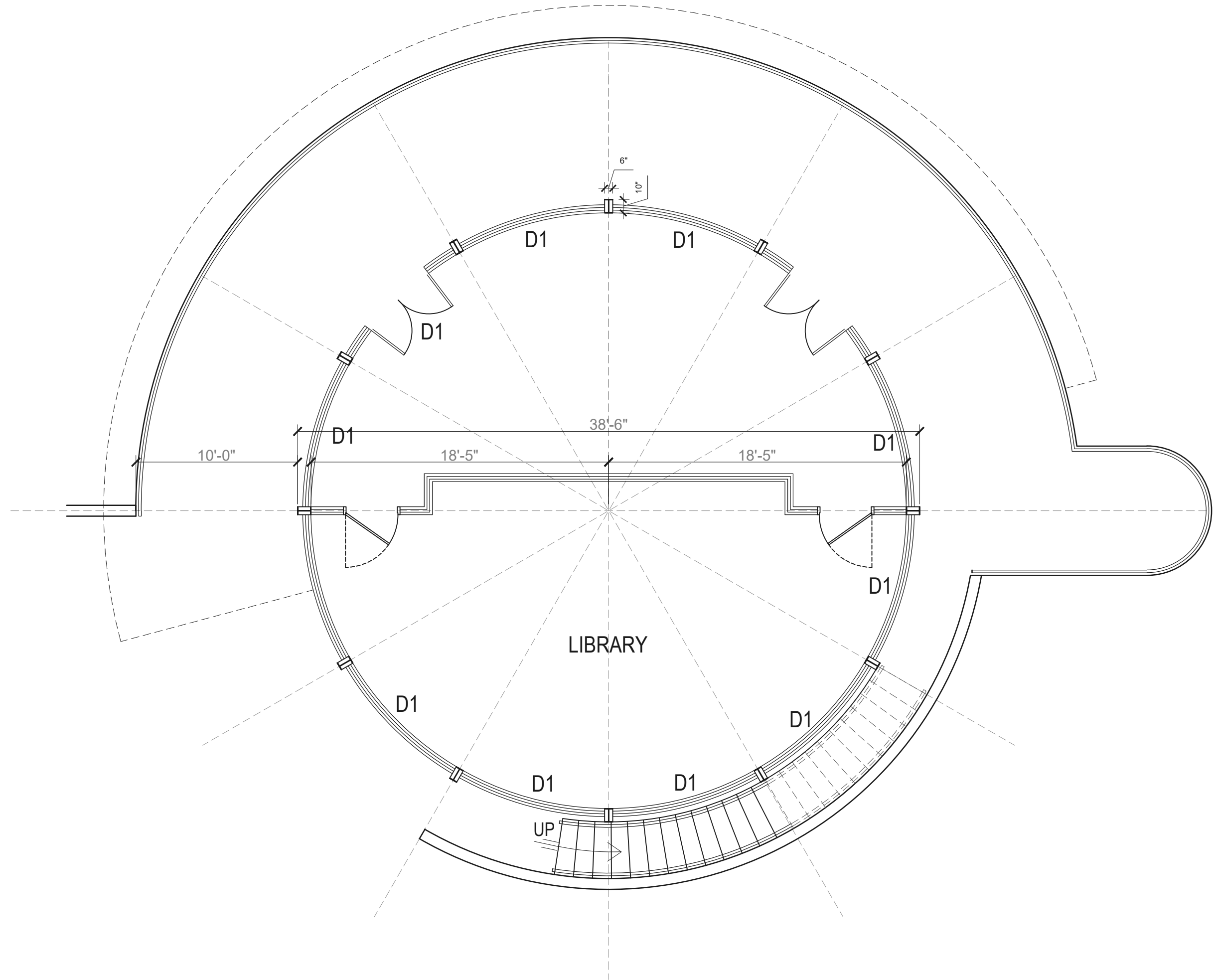
GROUND FLOOR PLAN SCALE = 3/8" = 1'-0"
